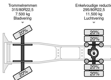
DAF 95.480 XF SPACECAB (EURO 3 / ZF16 MANUAL ... 4x2
