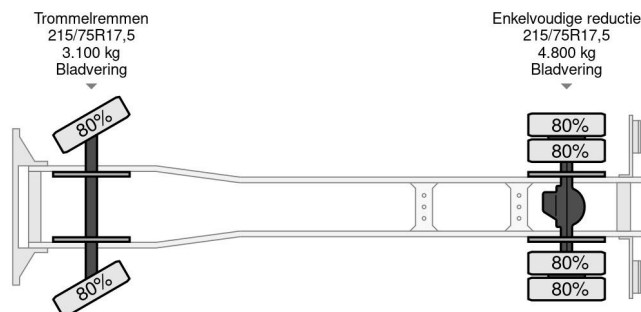
Mercedes-Benz LK 814 (6-CILINDER) FULL STEEL SU... 4x2
