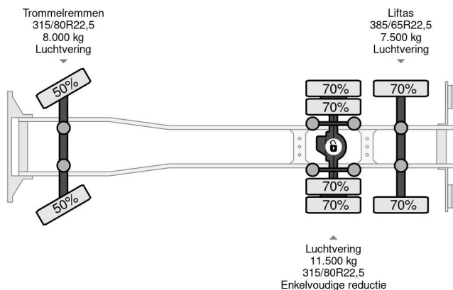
Scania R113-380 ML TOP-/STREAMLINE 6x2 HOOK-ARM (1... Referenznummer: SN 59459275
