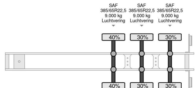
Schmitz Cargobull SCS 24/L 3-AXLE FLATBED TRAILER (D... Referenznummer: SN 60355362
