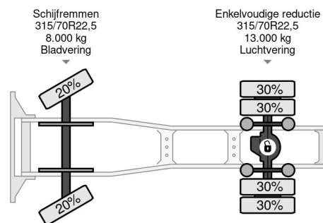
Iveco Stralis AS440S50T/P ACTIVE SPACE (EURO 5 / ... 4x2
