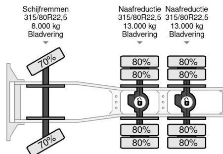
MAN TGA 33.460 BBS FULL STEEL SUSPENSION (ZF... 6x4 Referentienummer: SN 58659585
