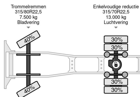
Scania R114-380 LA SLEEPERCAB 4x2 (EURO 2 / MANUAL...
