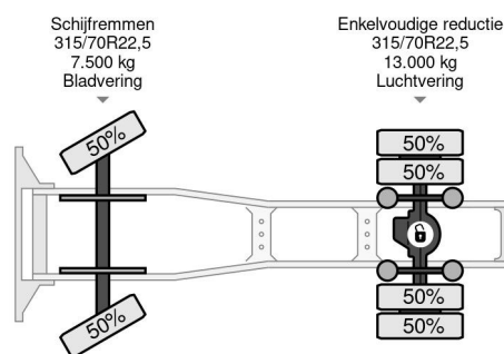
DAF XF 105.460 SPACECAB (ZF16 MANUAL GEARBOX / MX-BRAKE / 870+430 LITER TANK / FRIDGE / AIRCONDITIONING) 4x2
