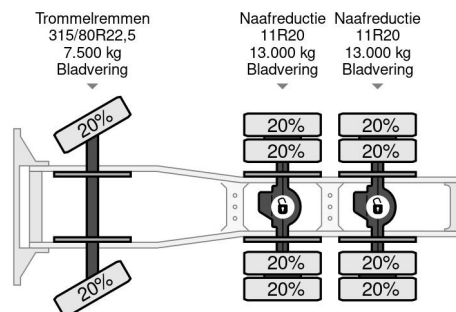
MAN 26 240DFS FULL STEEL SUSPENSION / DAYCA... 6x4
