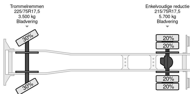
Mercedes-Benz LK 914 4x2 FULL STEEL CHASSIS (6-CILIN...
