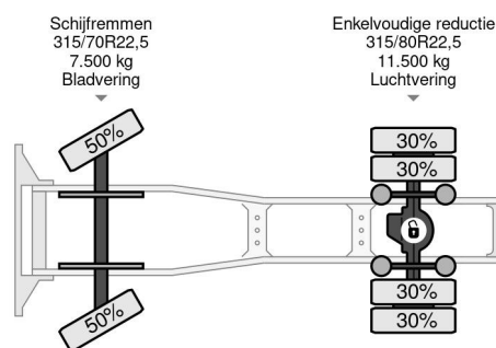
Renault Magnum AE 440 E-TECH (MACK ENGINE / ZF... 4x2
