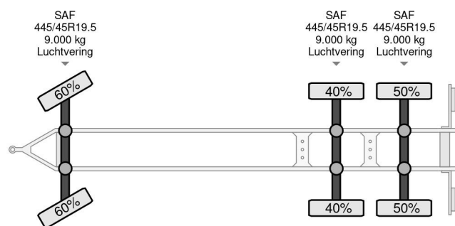
Burg BPA09-18AC 3-AXLE CONTAINER HANGER (SAF AXL...
