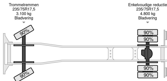
Mercedes-Benz LK 814 K 6-CILINDER FULL STEEL WI... 4x2
