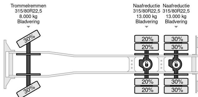
Volvo FM 10.360 6x4 FULL STEEL KIPPER (REDUCTION A...
