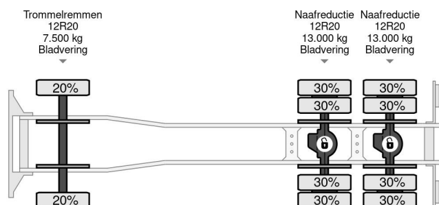
Mercedes-Benz SK 2527 K 6x4 FULL STEEL CHASSIS (MA... Referentienummer: SN 53127228
